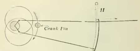
FIG. 11. DIRECT MOTION—NO ROCKER.
